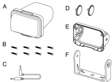
Figure 1. Parts of SM-200. (A) SM-200 audio housing (B) mounting screw \times 8 (C) audio cable with 3.5mm 4-pin plugs (D) thumbwheel screw \times 2 (E) housing holder (F) Bracket
