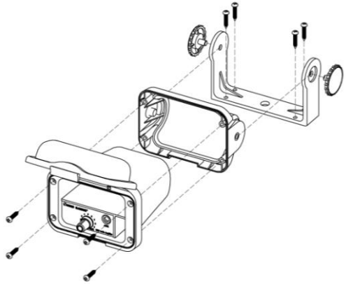
Figure 5. A summary of SM-200 installation.
