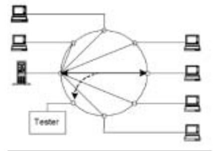
Figure 5 – Logical effect of configuring a mirror port.
