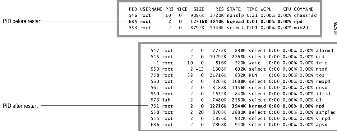
Figure 14: Restarting a Process
