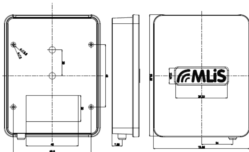
Figure 2: Chassis Dimension for MLB-G3002
