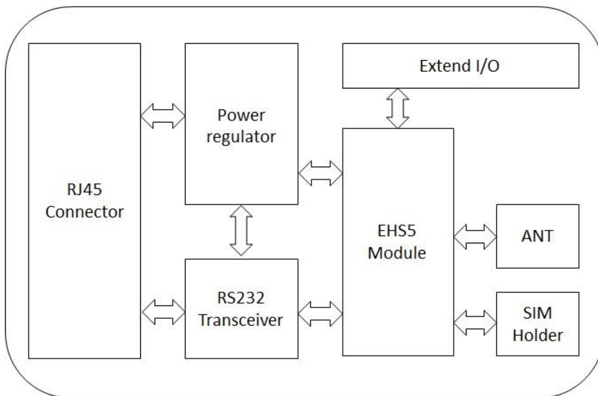
Figure 1: Functional Block Diagram for MLB-G3002
