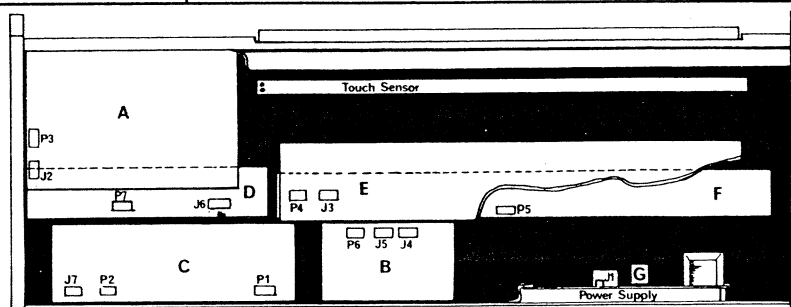
2701 BOARD LOCATIONS
