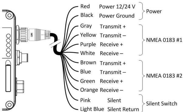
Figure 2 Wiring instructions
