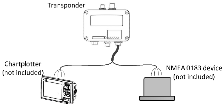
Figure 3 Multiplexing with NMEA0183 ports
