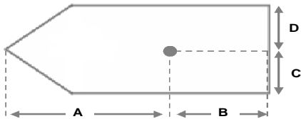
Figure 3 GPS antenna location
