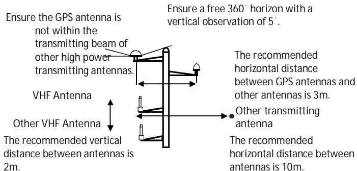
Figure 2 VHF/GPS antenna locations
