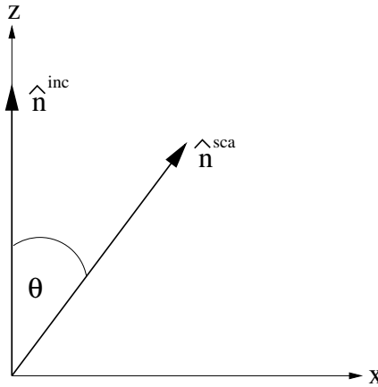
Figure 8.1: Illustration of the scattering frame. The z-axis coincides with the incident direction \hat{\mathbf{n}}^{\text{inc}} . The scattering angle \Theta is the angle between \hat{\mathbf{n}}^{\text{inc}} and \hat{\mathbf{n}}^{\text{sca}} .
