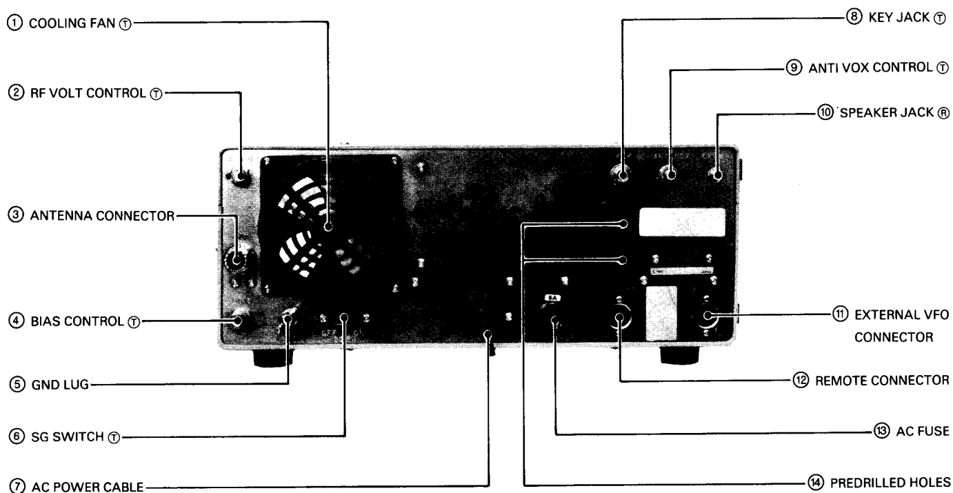
Fig. 3-2 Rear Panel View
