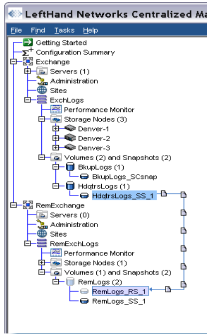
Figure 2.4. Remote copy in progress
