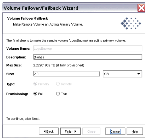
Figure 2.22. Making the remote volume into an acting primary volume
