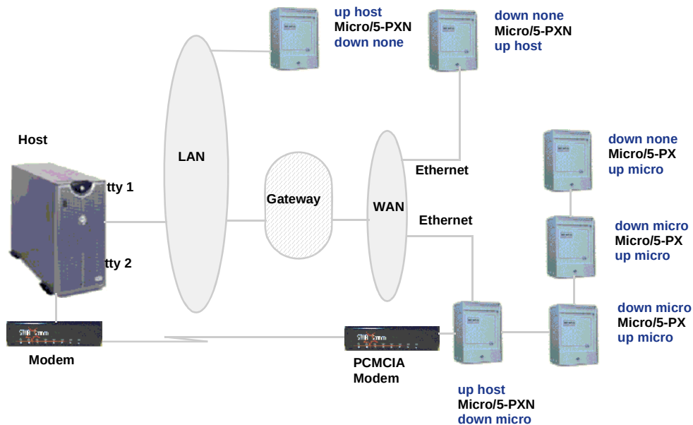
Figure 54. Sample Ethernet configuration
