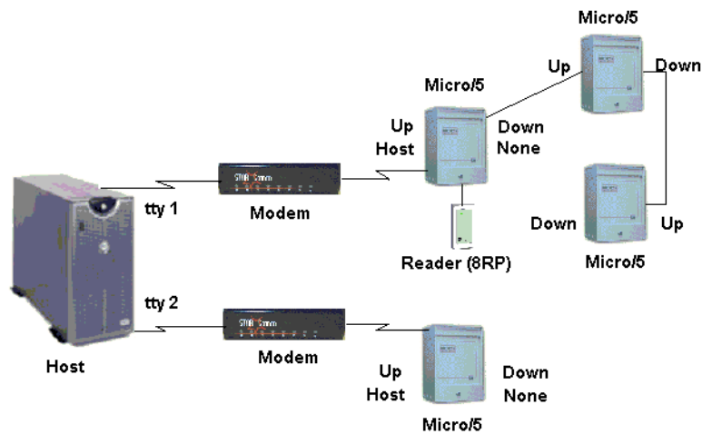
Figure 53. Example of Dial-up communication
