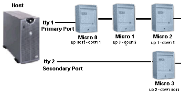
Figure 52. Example of direct communication - Bi-directional micros
