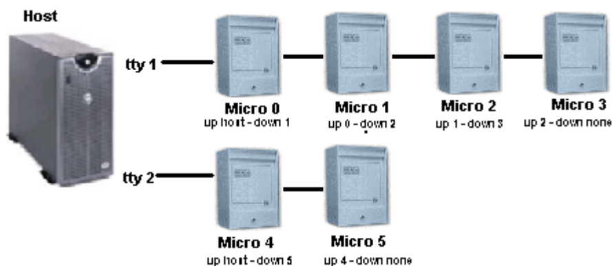
Figure 51. Example of direct communication - Uni-directional micros
