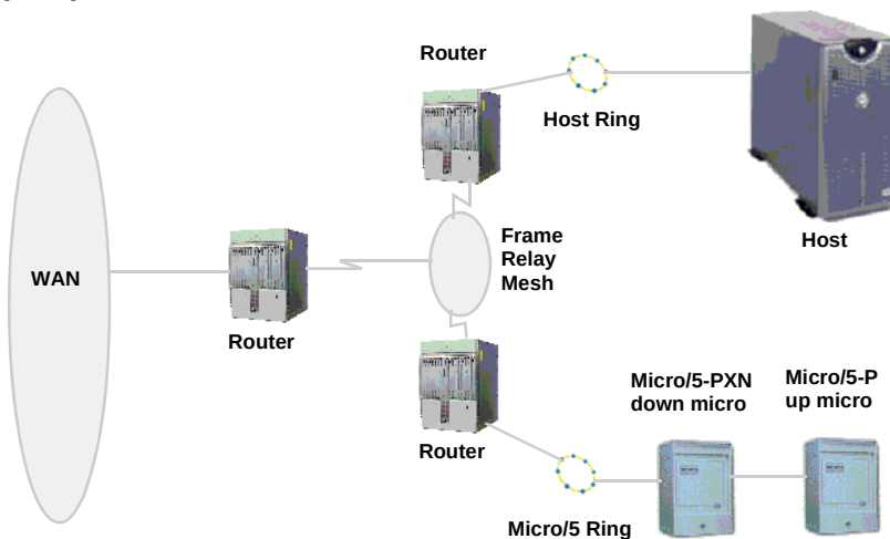
Figure 55. Sample Token ring configuration
