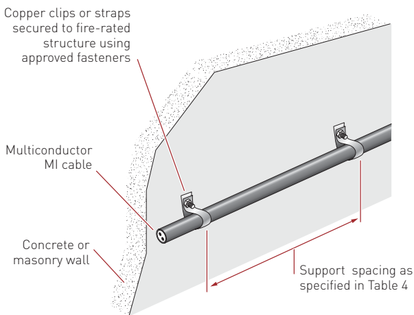
Figure 25: Typical surface-mounted installation using clips or straps
