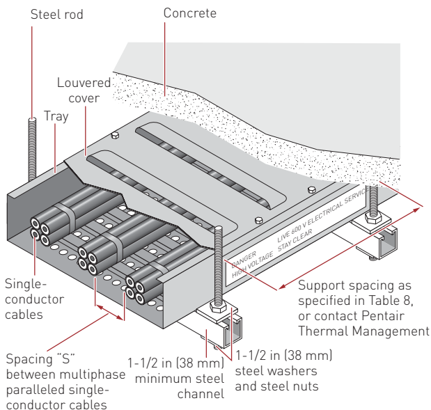
Figure 36: Typical service entrance installation with tray mounted on steel trapeze
