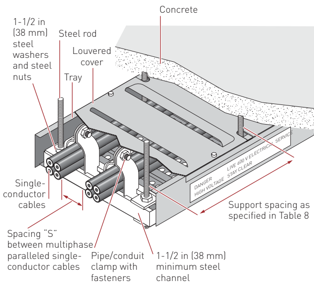
Figure 37: Typical service entrance installation with steel trapeze mounted inside cable tray
