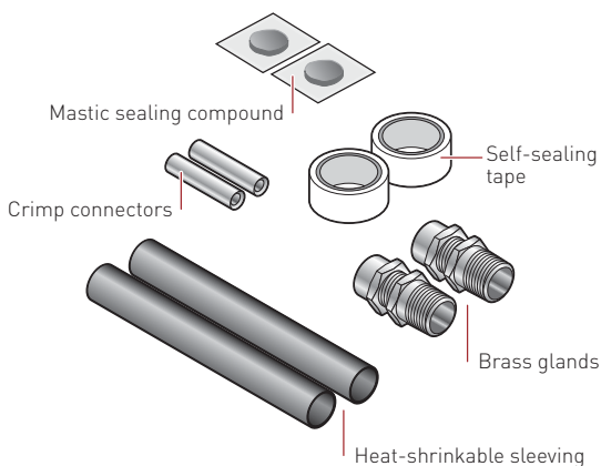
Figure 38: System 1850-SE termination kit
