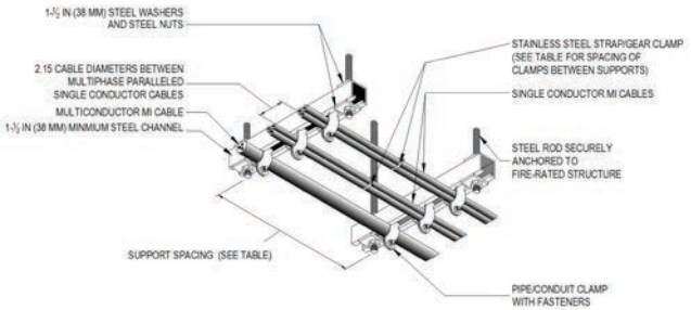
Figure 5: Steel strut trapeze
