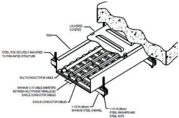
Figure 6: Cable tray
