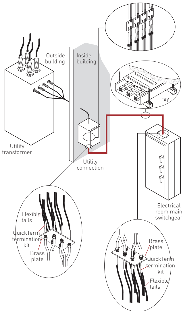
Figure 34: Typical System 1850-SE power circuit
