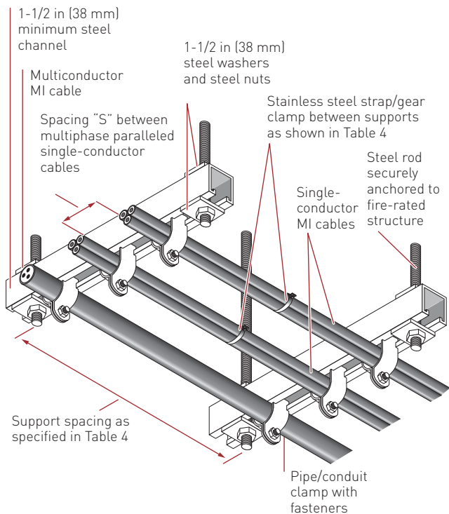
Figure 22: Typical installation using trapeze support – alternate method
