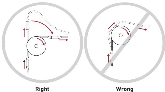
Figure 29: Procedure for pulling factory-installed joints
