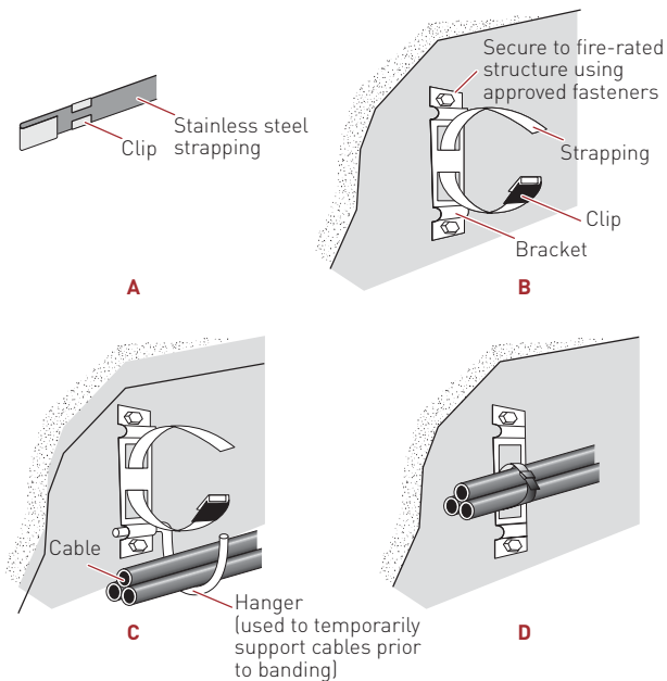
Figure 26: Banding bracket installation
