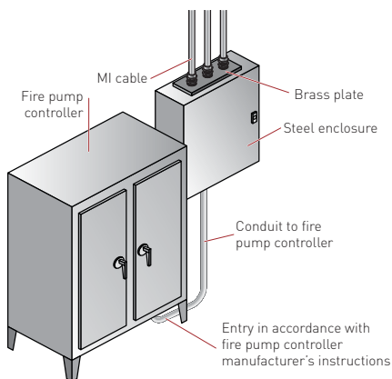
Figure 12: Brass plate installation
