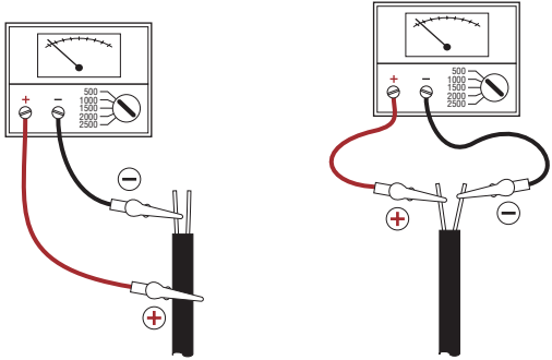
Figure 39: IR test between cable sheath and conductor and between conductor pair
