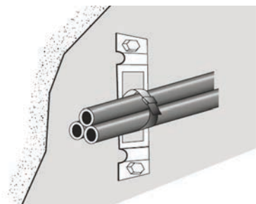
Figure 1: Steel banding and bracket
