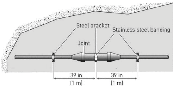
Figure 7: Splice - Factory Joint
