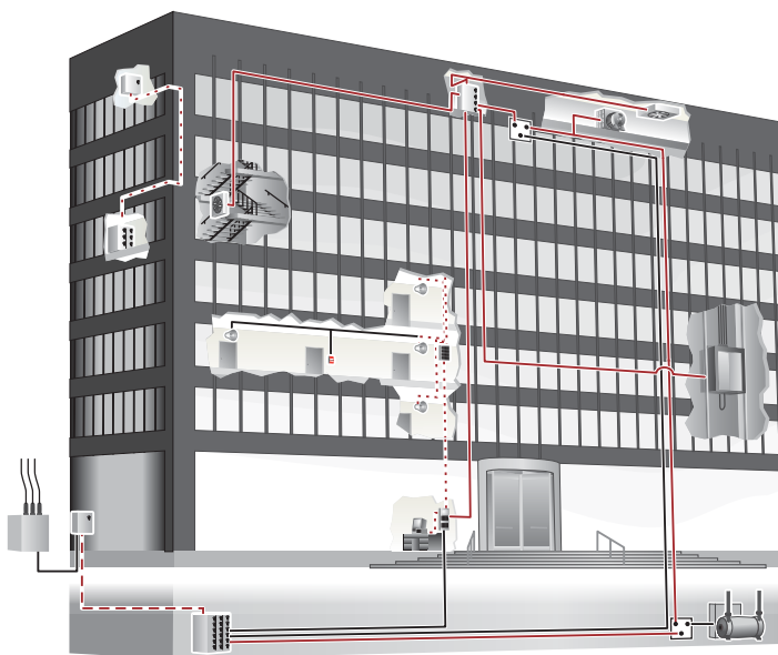
Figure 2: Typical MI cable application
