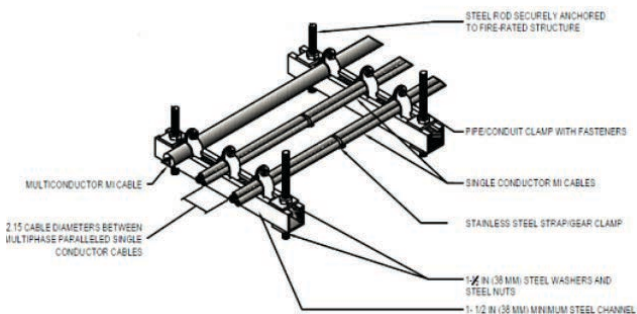
Figure 4: Steel strut trapeze
