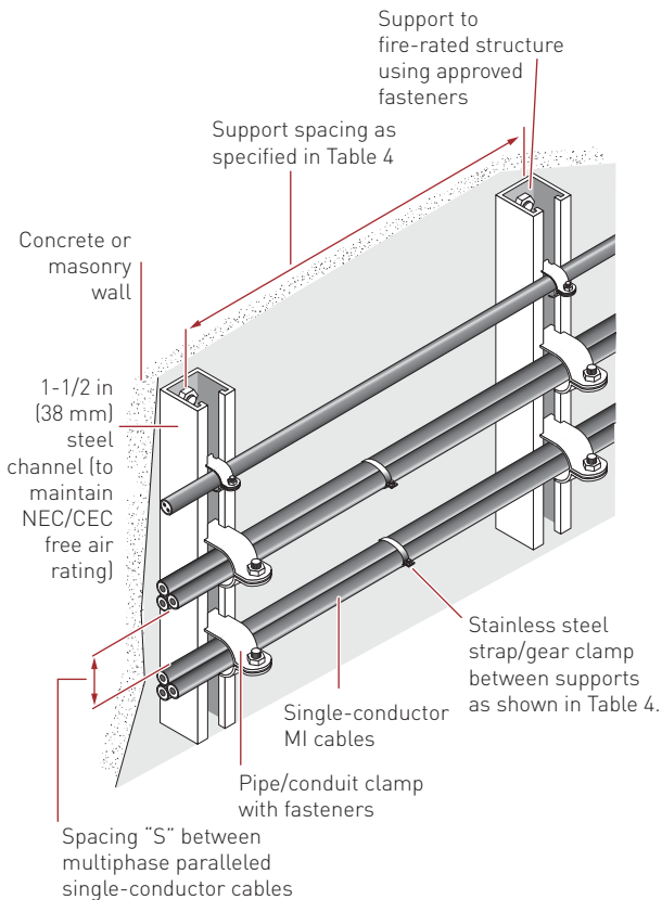
Figure 23: Typical horizontal surface-mounted installation using steel channel
