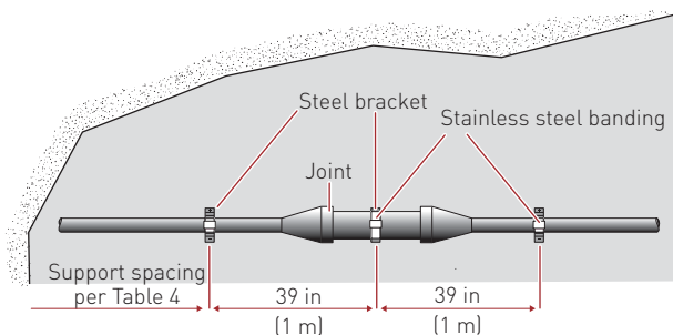
Figure 30: Supporting the factory-installed joint
