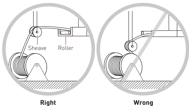
Figure 7: Reel setup
