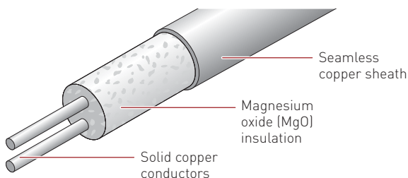
Figure 1: Pyrotenax MI cable
