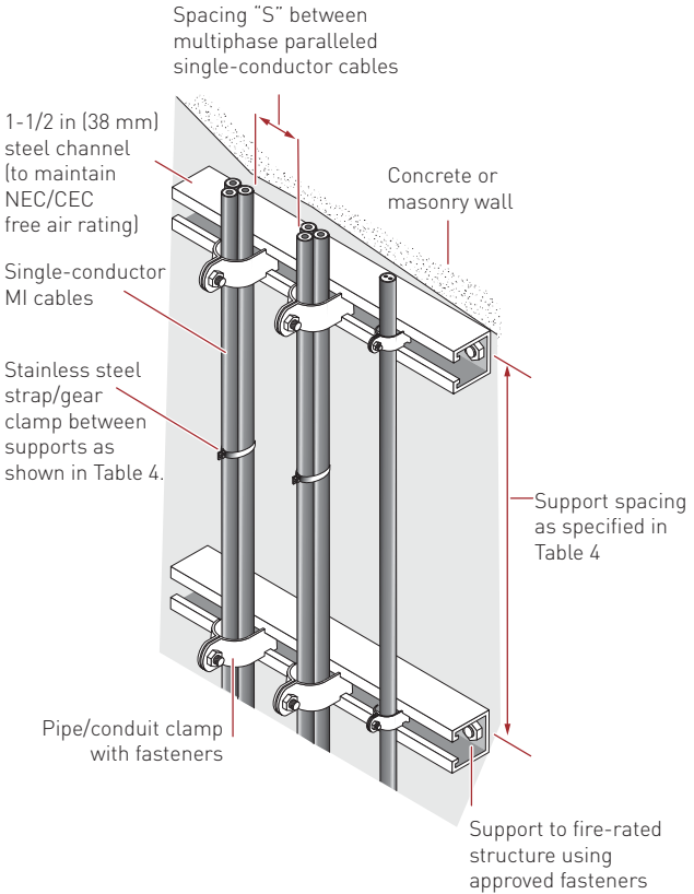
Figure 24: Typical vertical surface-mounted installation using steel channel
