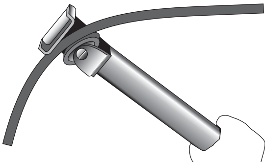
Figure 9: Bending MI cable
