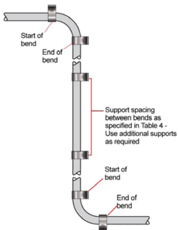
Figure 20: MI cable bends
