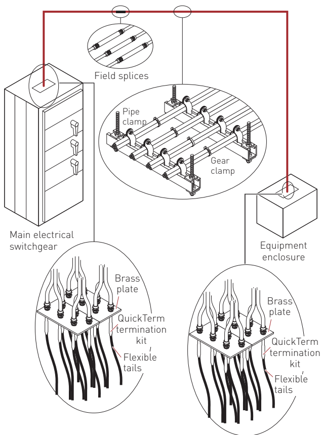
Figure 32: Typical System 1850 for Space Savings power circuit
