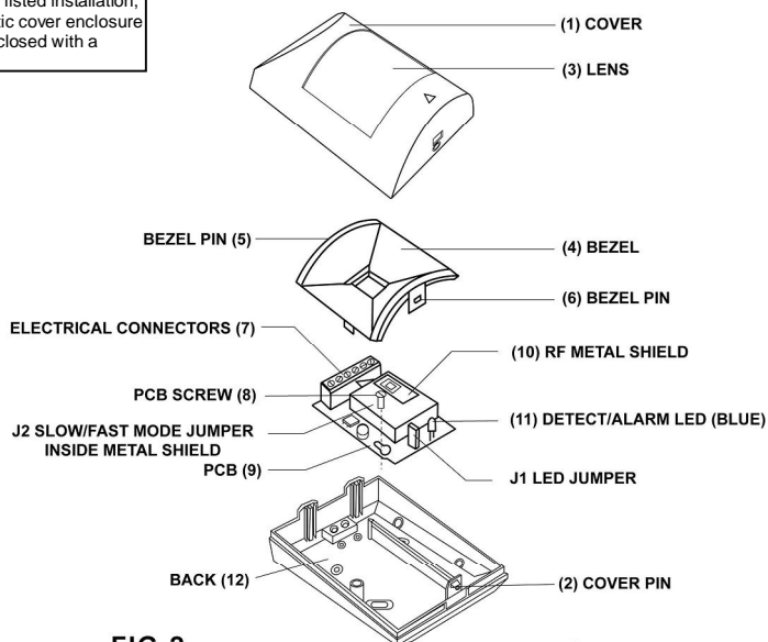
FIG-1 EXPLODED VIEW
