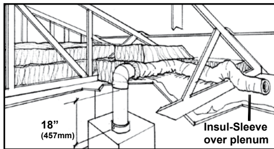
Fig. 02 - Attic Installation
