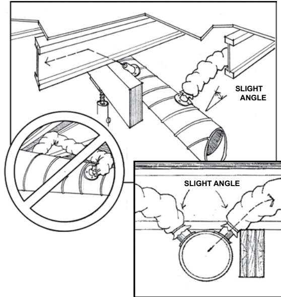
Fig. 18 - Secure to plenum with gentle bends
