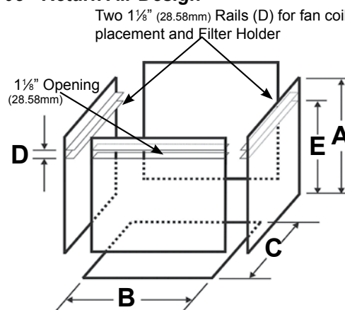
Fig. 03 - Return Air Design
