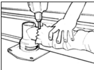
Fig. 19 - Mechanically Fasten
