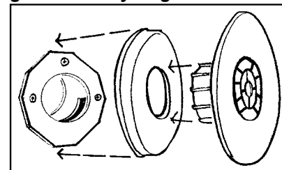
Fig. 32 - Beauty ring with Vent Plate
