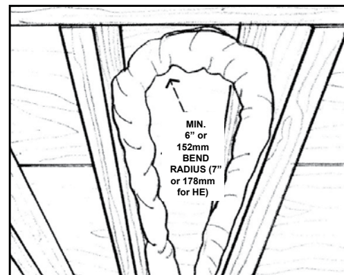
Fig. 17 - 6" (152mm) minimum radius on bends
