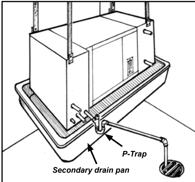
Fig. 03 - Secondary drain pan
