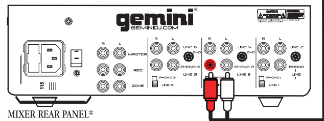
MIXER REAR PANEL*
