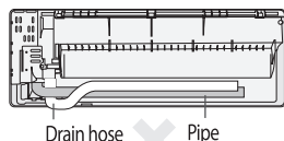
2) Incorrect connection
