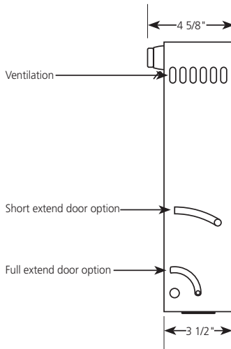
Figure 3-2. Side view.
