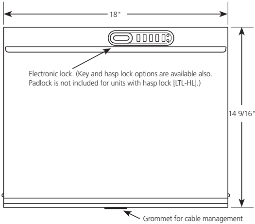
Figure 3-1. Front view.
