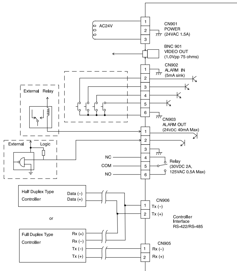
SCC-C6405(P) Adapter BOARD
