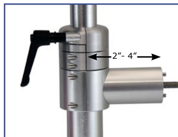
2" or 4" offset side mount allows mounting to any flat surface
