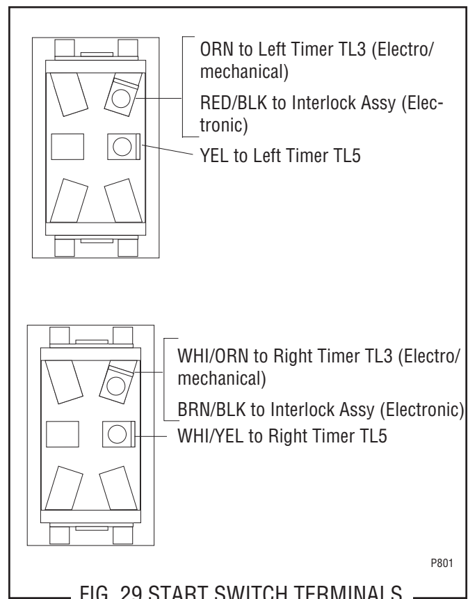
FIG. 29 START SWITCH TERMINALS
