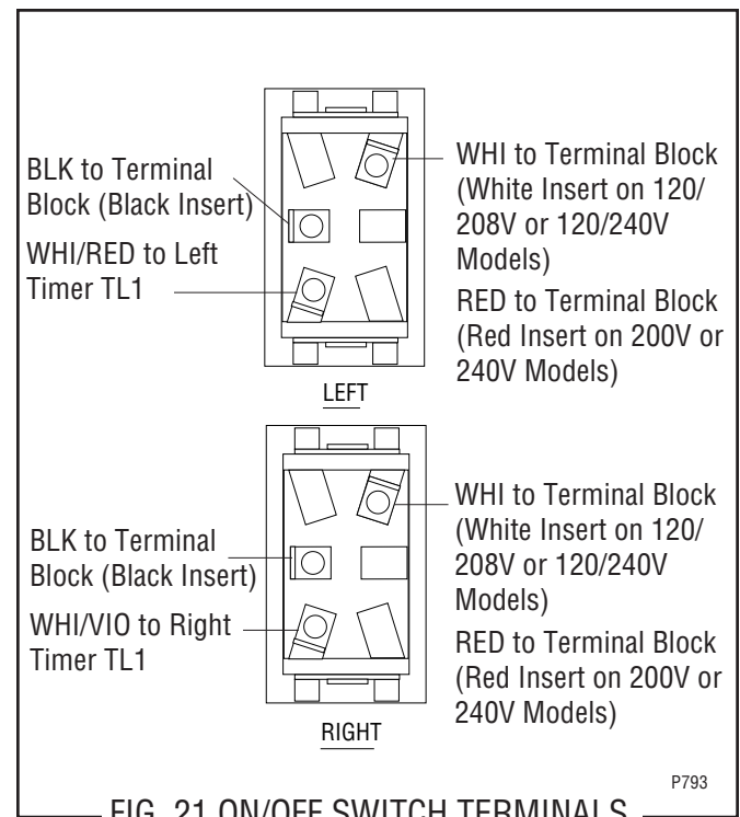
FIG. 21 ON/OFF SWITCH TERMINALS
