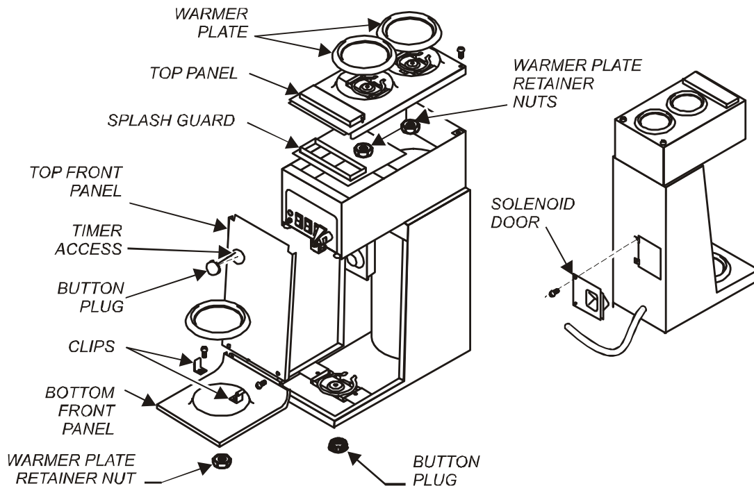
Fig. 9 Access Panels
