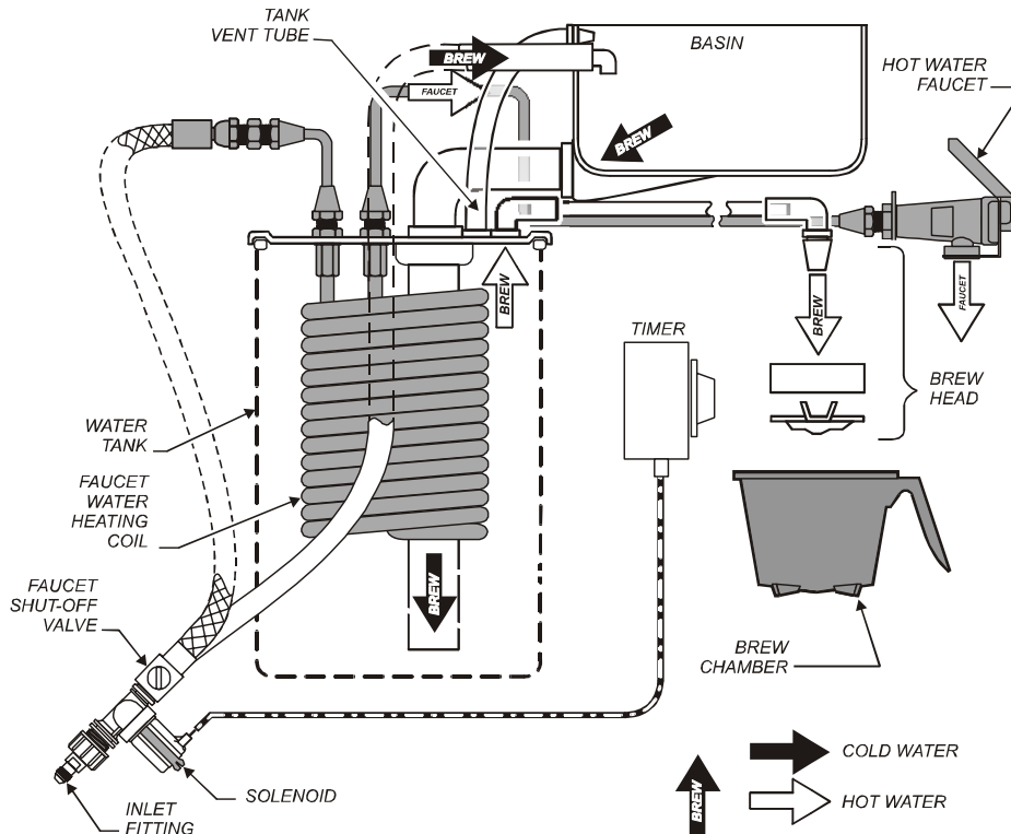
Fig. 4 Brewer Operation Diagram
