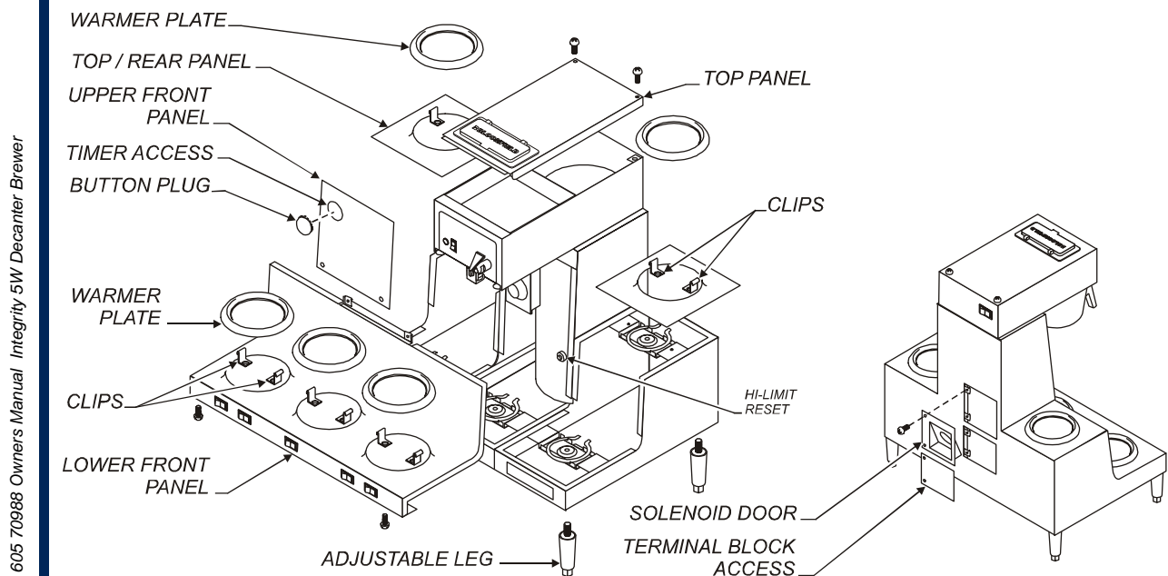
Fig. 9 Access Panels
