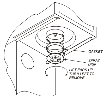
Fig. 8 Cleaning
