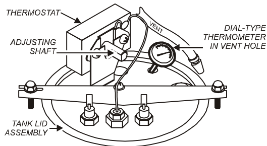
Fig. 10 Checking and Adjusting Brew Temperature
