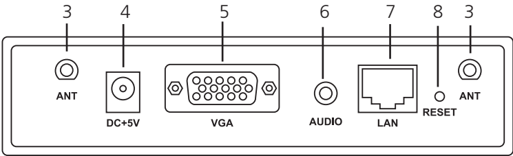
Figure 3-2. Back panel.
