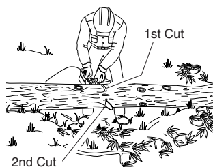
Figure 18 - Bucking Log When Log Is Supported On Both Ends
