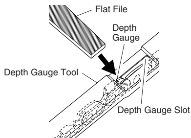
Figure 24 - Depth Gauge Tool On Chain
