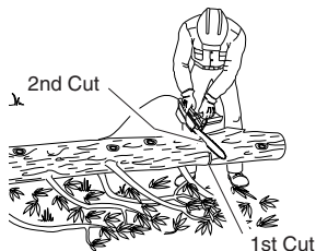
Figure 17 - Bucking Log When Log Is Supported On One End
