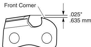
Figure 25 - Round Off Front Corner Of Depth Gauge
