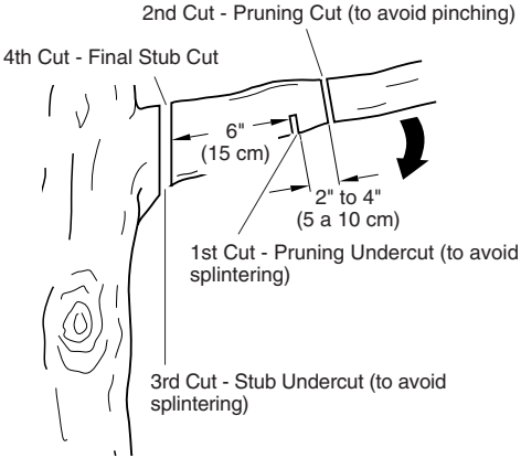
Figure 19 - Cutting A Limb
