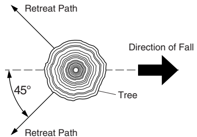
Figure 13 - Retreat Path From Tree
