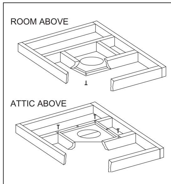
Figure 14A Installing the Firestop Spacer
