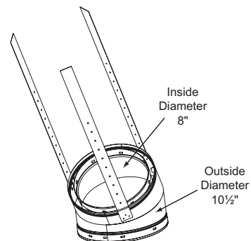
SL315-330 - Offset/Return
