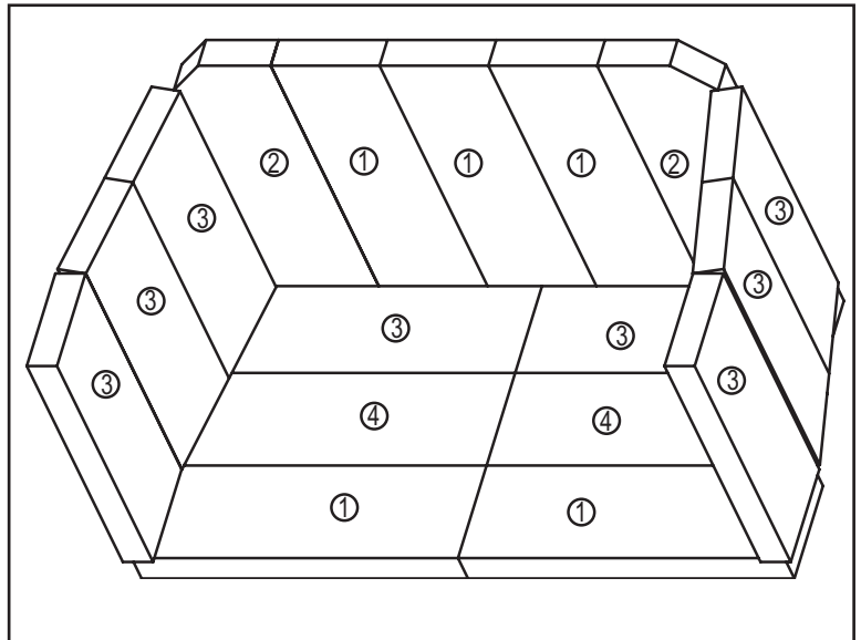
Figure 29A-Brick Pattern
