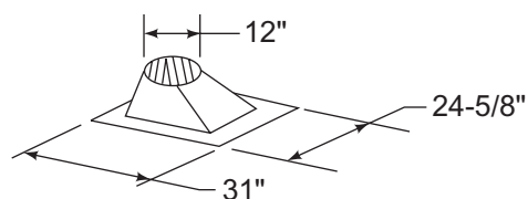
RF371 - Roof Flashing 6/12 to 12/12 Pitch
