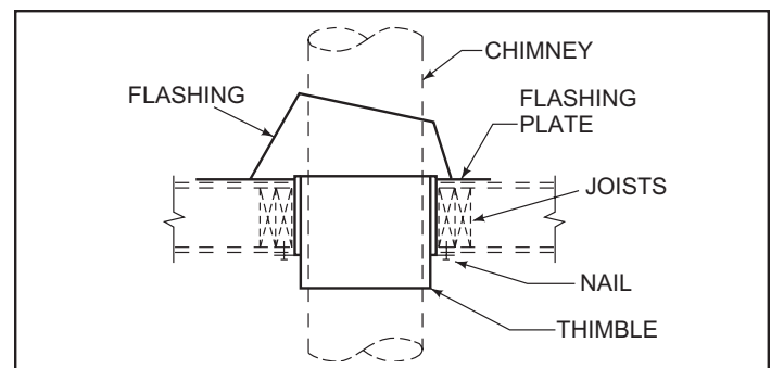
Figure 15A - Installing an MH842, Configuration 1
