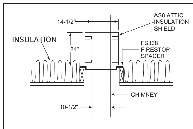
Figure 14B Installing an Attic Insulation Shield
