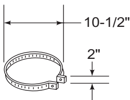
JB877 Joint Band
