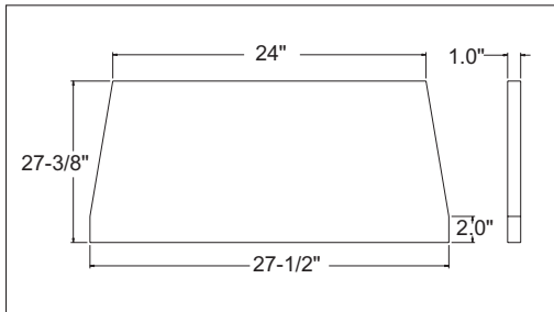
Ceramic Blanket
