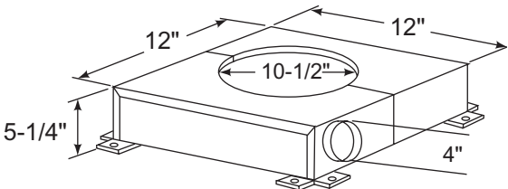
CAK4A Chimney Air Kit
