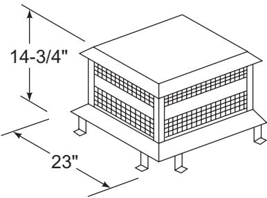
ST375 Square Termination Cap
