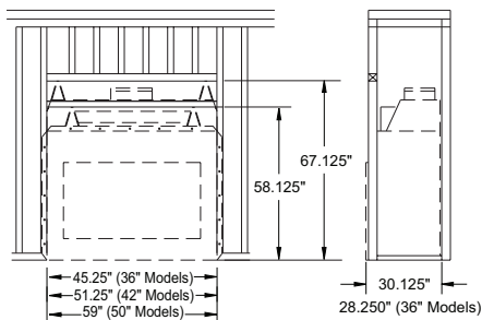
Figure 4 - Framing Dimensions
