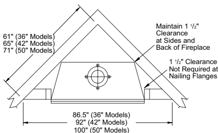
Figure 5 - Corner Installation
