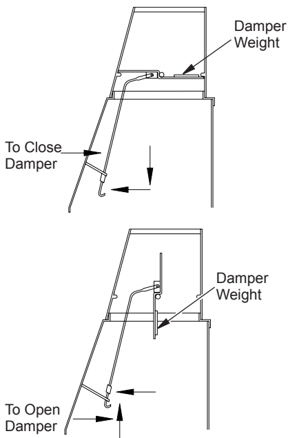
Figure 32 - Operating Damper Handle
