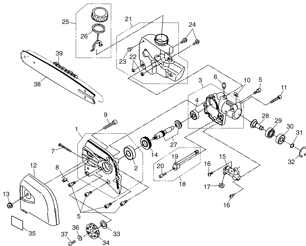
Fig.2 CUTTING UNIT PSZ2401/PSZ2401-CA (S/N 000000 and up)
