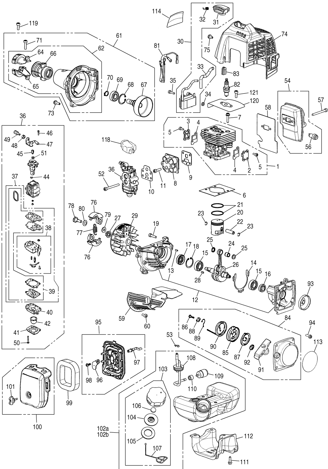
Fig.3 ENGINE UNIT PSZ2401/PSZ2401-CA (S/N 60600101 and up)
