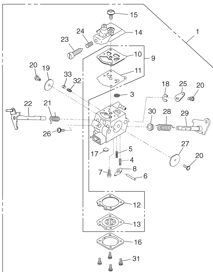
Fig.3 CARBBURETOR COMPONENTS (S/N 600101 and up)
