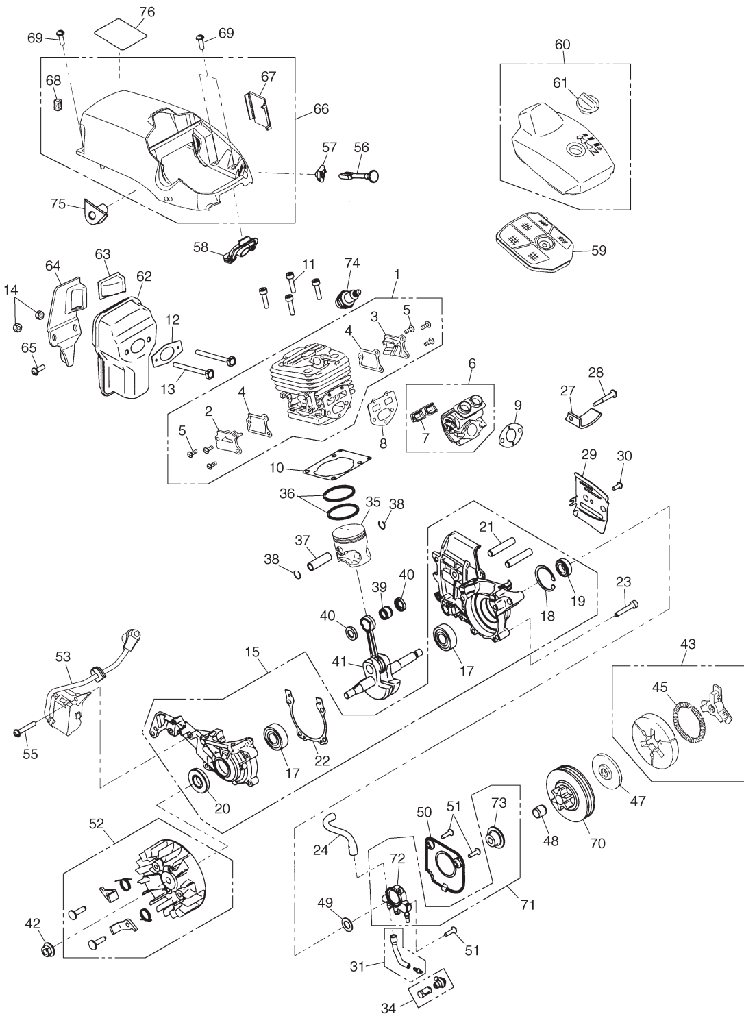
Fig.1 POWER UNIT (S/N 600101 and up)
