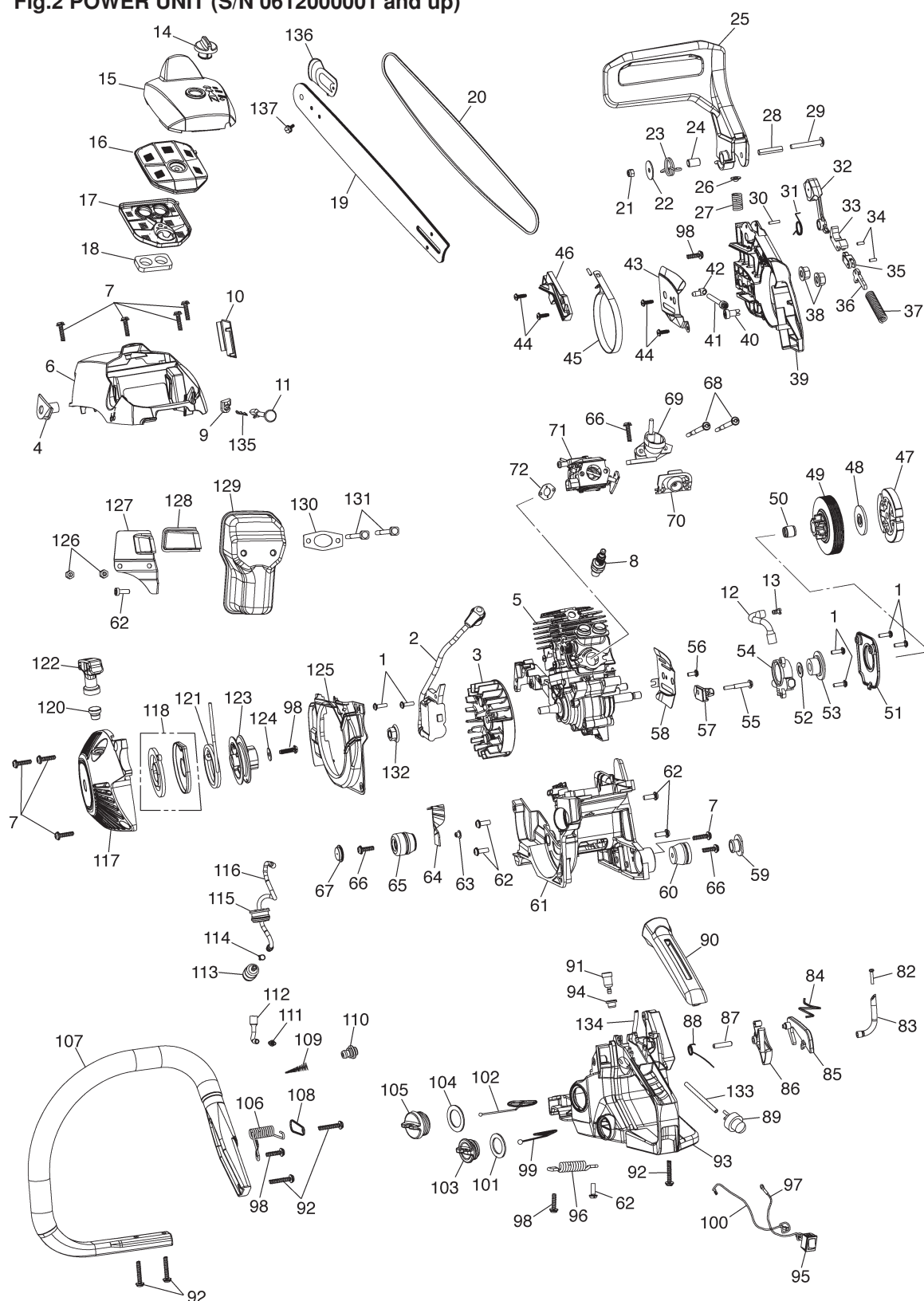
Fig.2 POWER UNIT (S/N 0612000001 and up)
