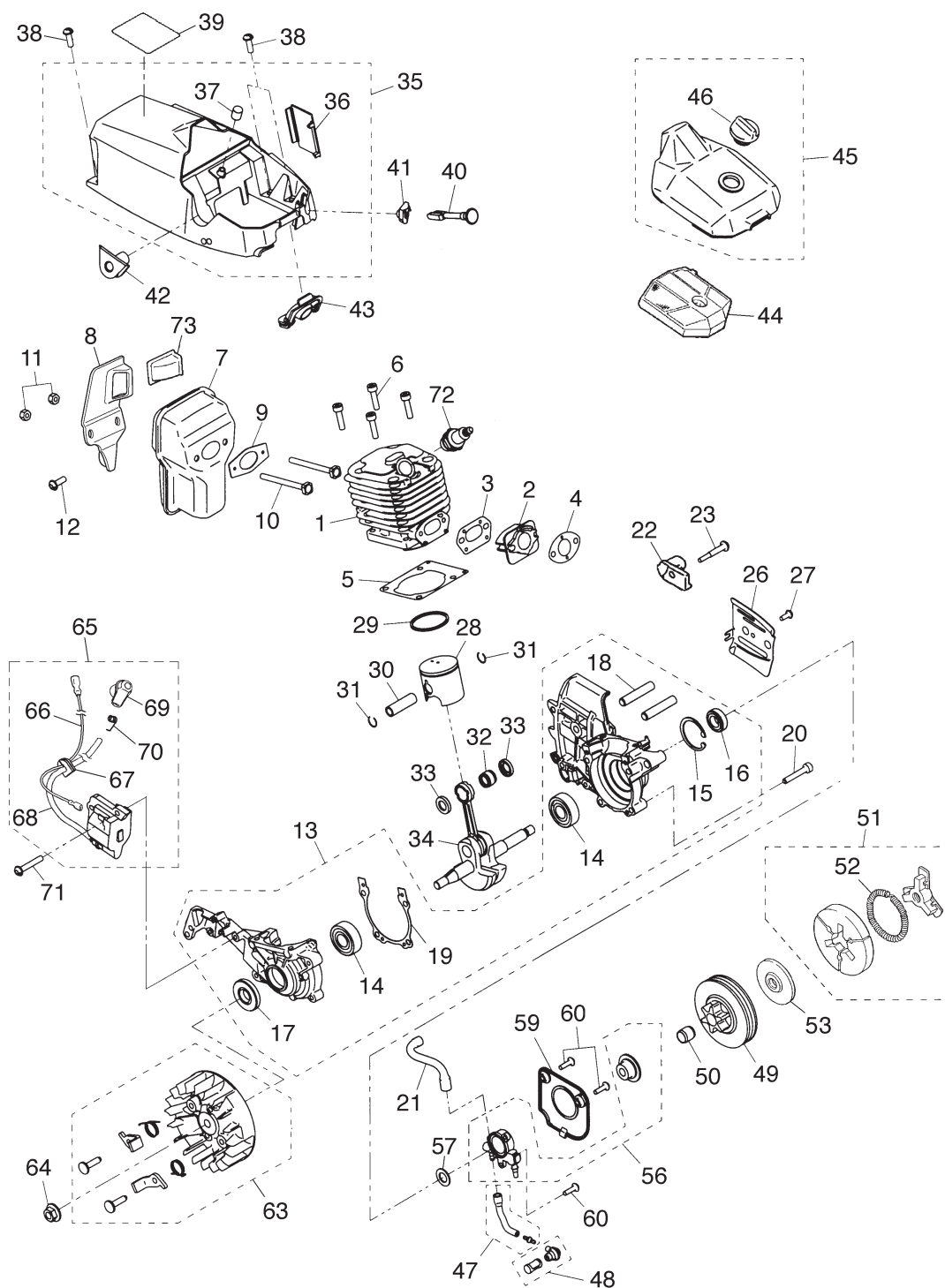
Fig.1 POWER UNIT (S/N 793480 and up)
