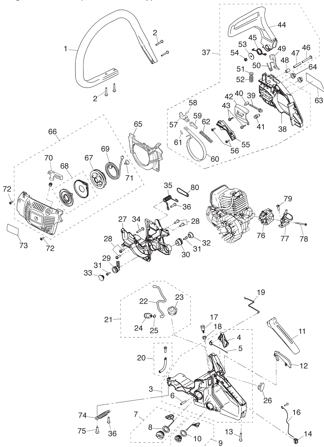
Fig.2 POWER UNIT (S/N 793480 and up)
