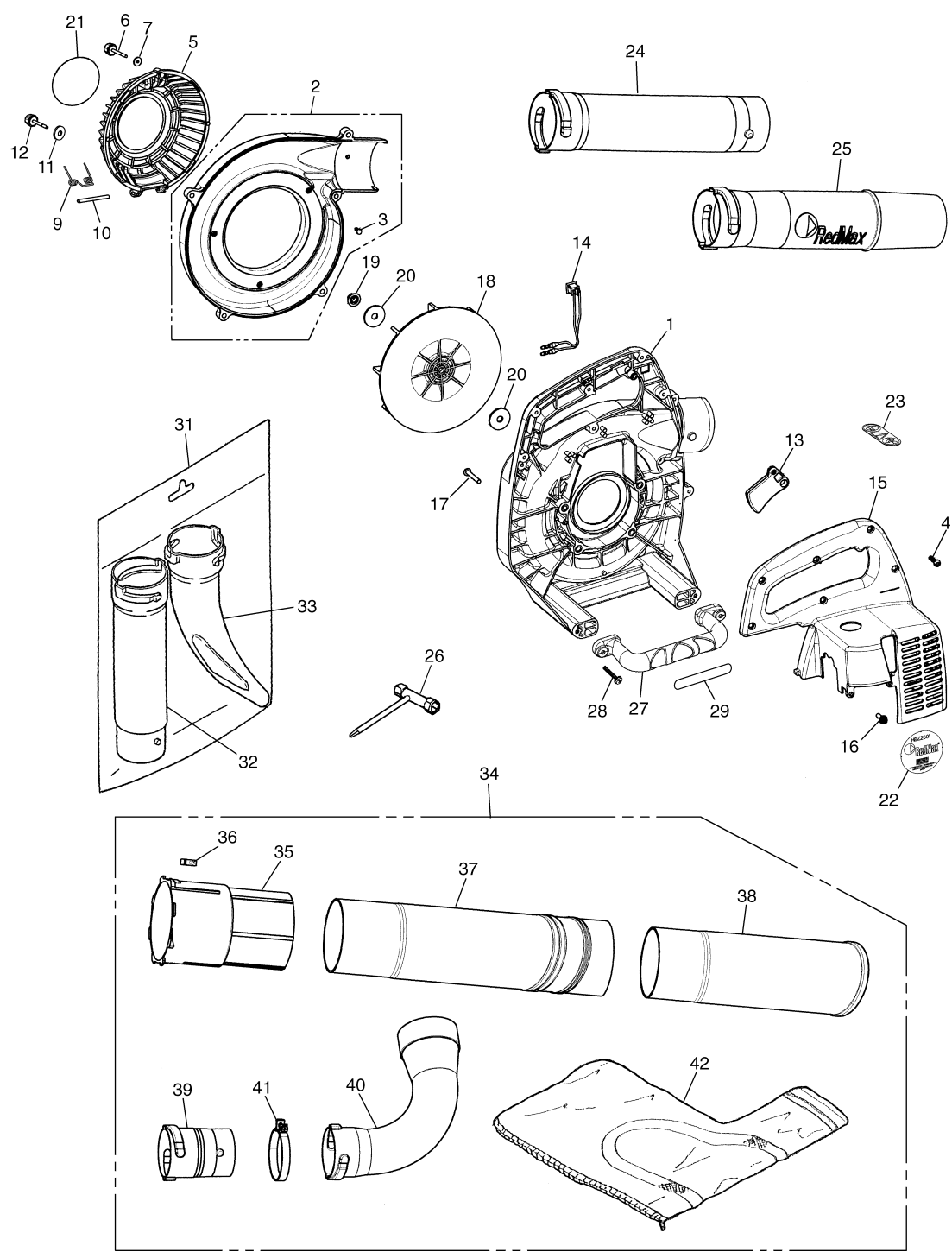
Fig.2 BLOWER GROUP HBZ2601/HBZ2601-CA
