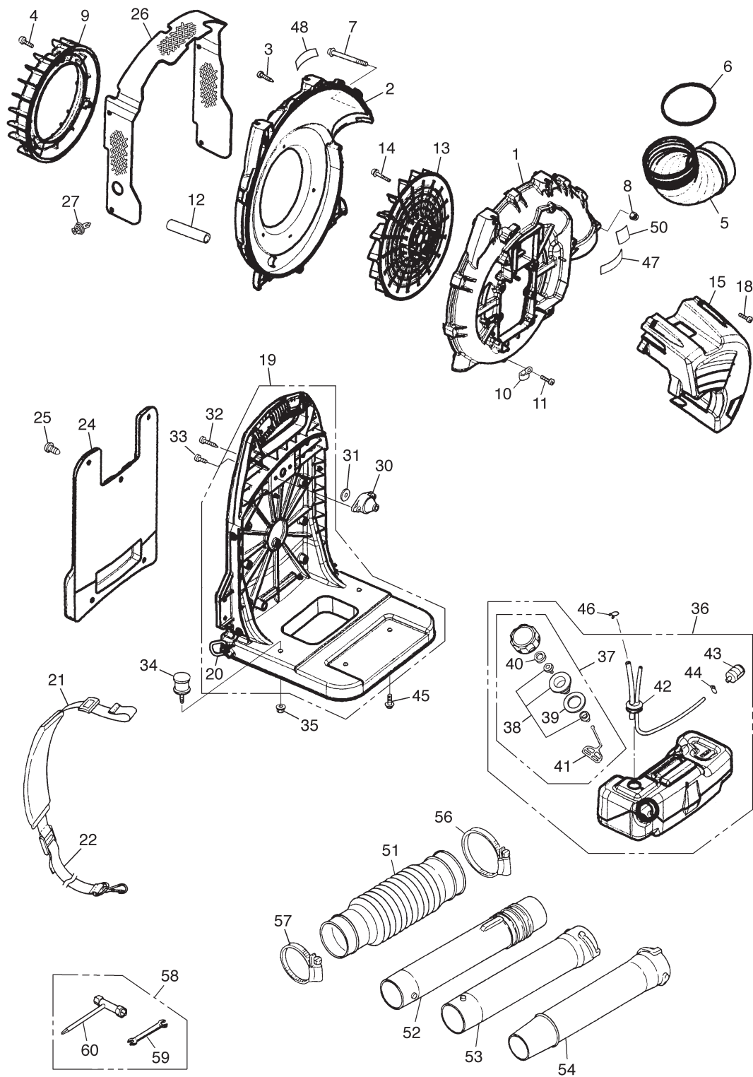
Fig.1 BLOWER GROUP (S/N 300001 and up)
