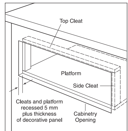
Recessed cleats and platform – inset application
