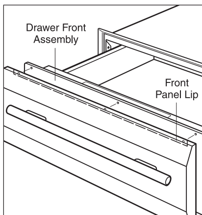
Attach handle
