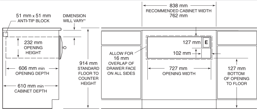
Undercounter Installation – Stainless Steel Drawer Front
