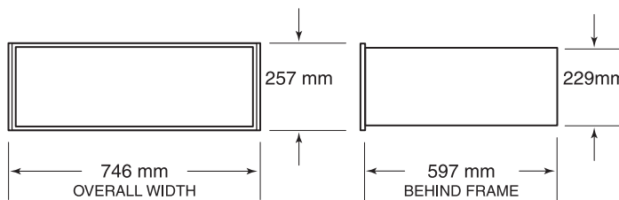
Overall Dimensions – Integrated Drawer Front
