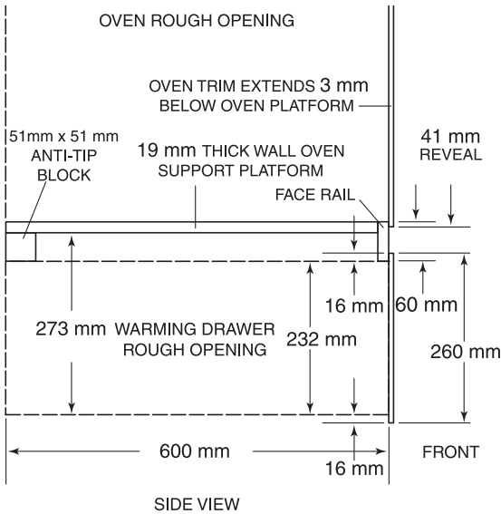
Installation with Built-In Oven – Stainless Steel Drawer Front
