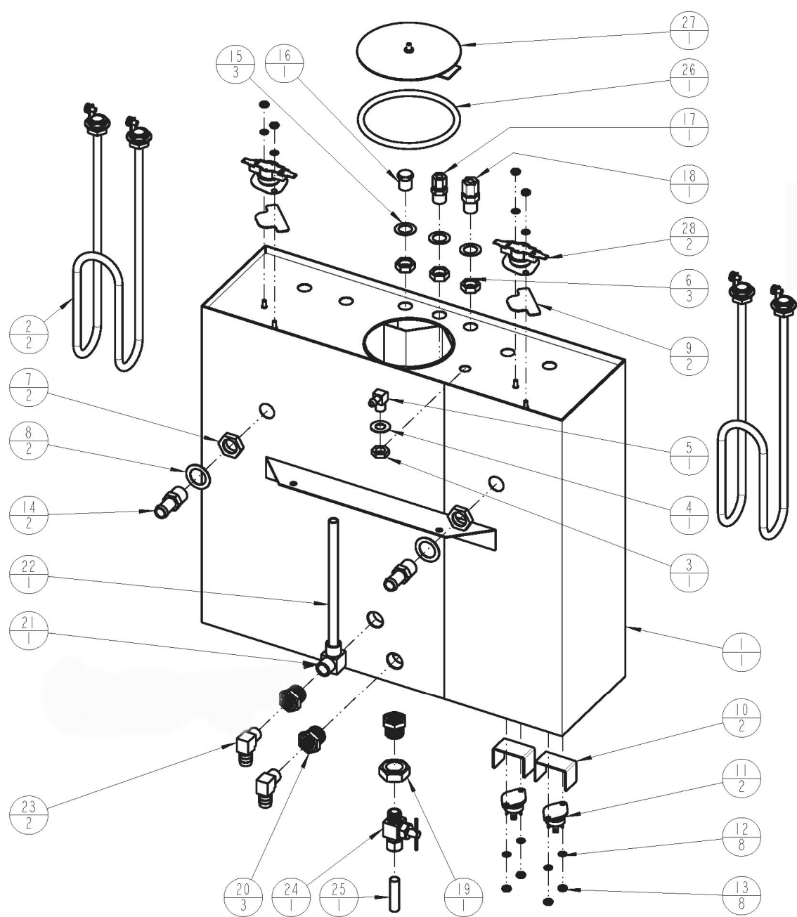
Figure 4 – CBS-2032e / CBS-2032s Tank Assembly
