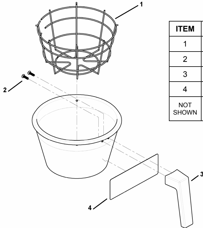
Figure 6 – Brew Basket Assembly, 13” X 5”, Part # 101171 (ROUND)
