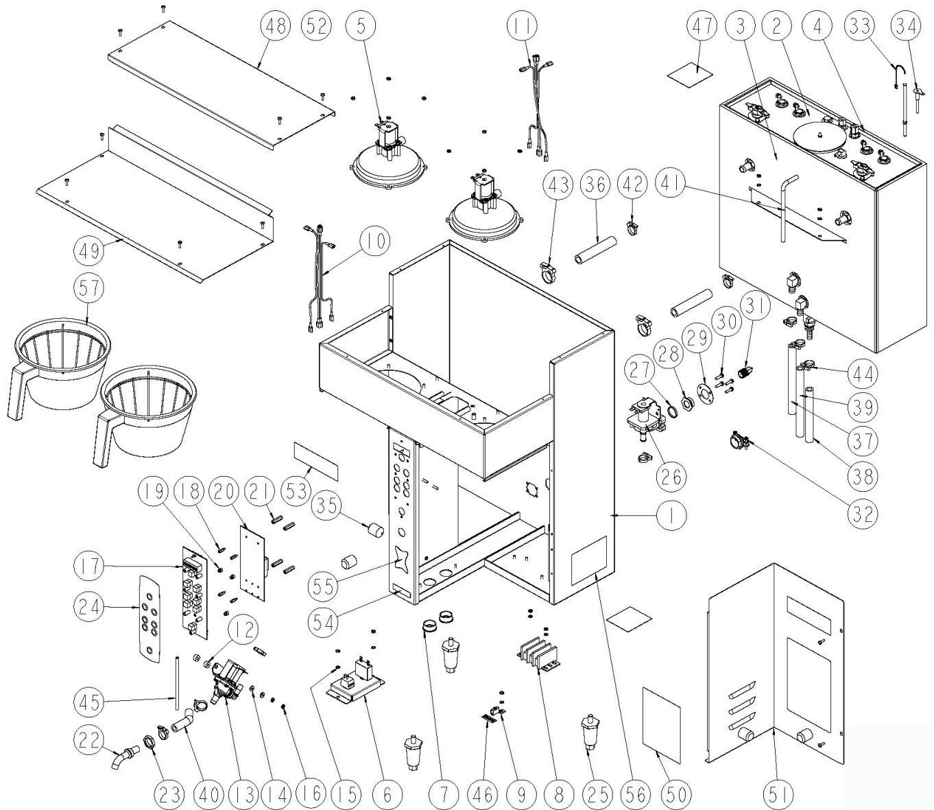
Figure 3 – CBS-2032e / CBS-2032s Main Assembly
