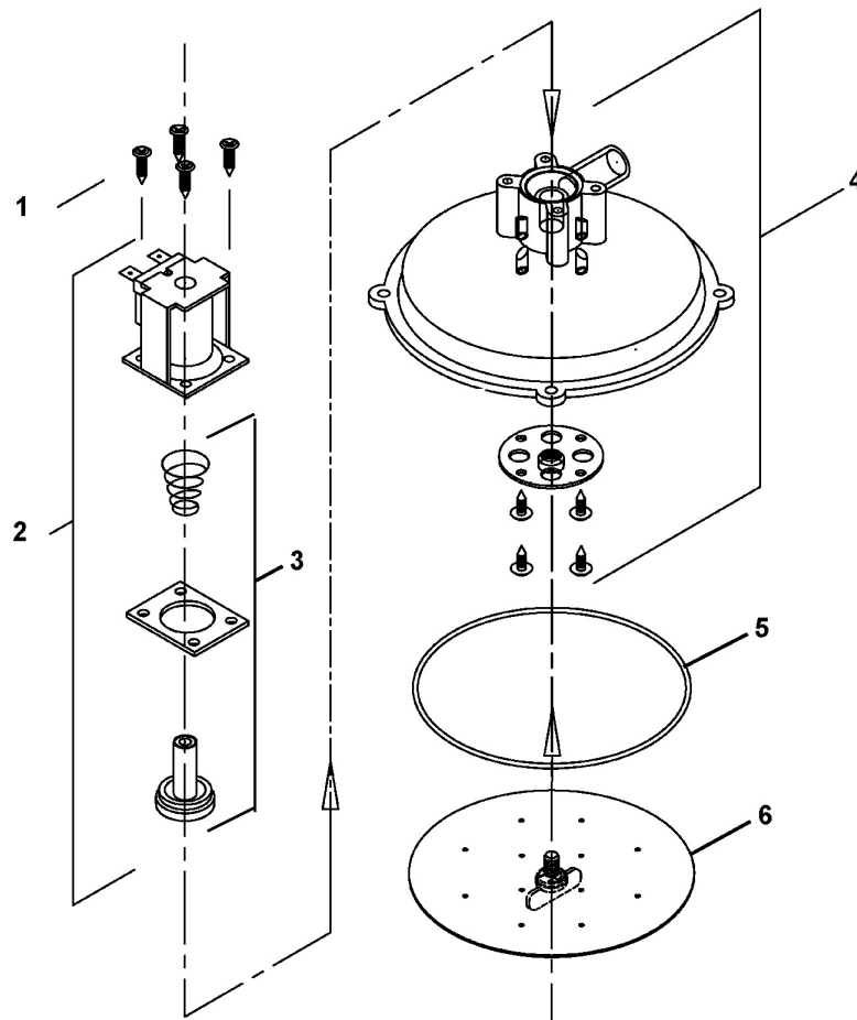
Figure 5 – Spray Housing Assembly, 120 VAC, Part # 102080 Spray Housing Assembly, 220 VAC, Part # 102158 (EXPORT ONLY)
