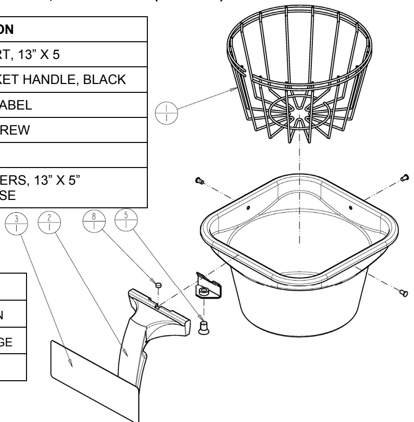
Figure 7 – Brew Basket Assembly, 13” X 5”, Part # 101175 (SQUARE)
