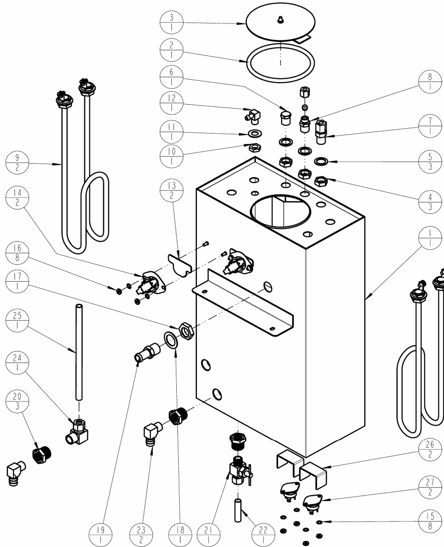
Figure 2 – CBS-2031e / CBS-2031s Tank Assembly
