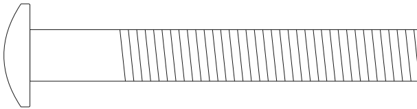
M10 x 75 Bolt Quantity: 4
