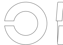
12.2 x 21.5 x 3 Lock Washer Quantity: 4
