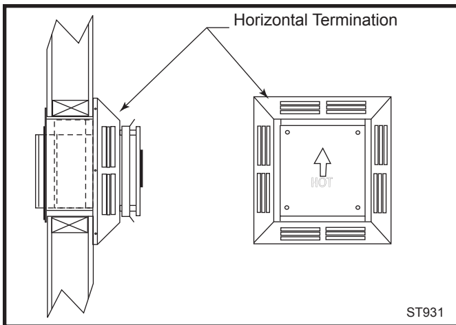
Fig. 41 Horizontal termination.
