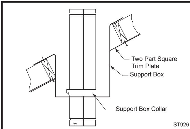
Fig. 36 Support box.
