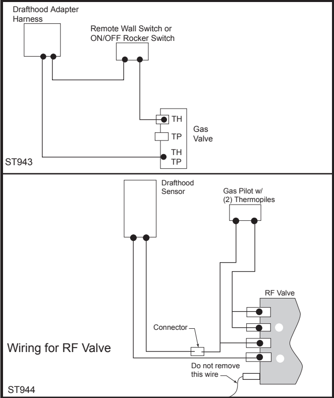
Fig. 80 Draft hood adapter wiring. 20012734
