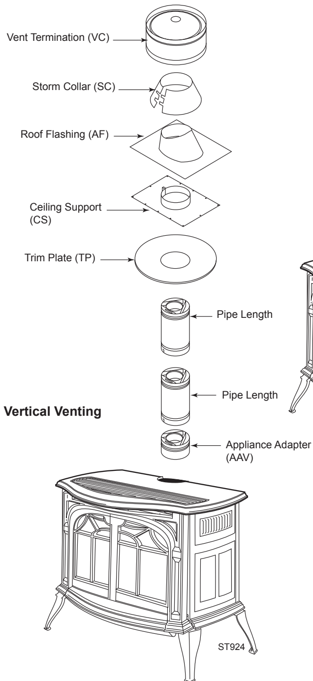
Fig. 34 Selkirk Venting Components
