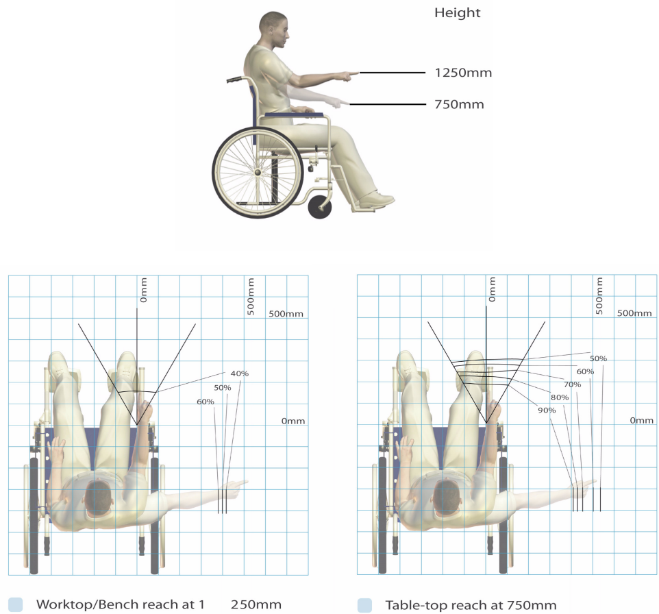
Figure 10 Reach Contours (Wheelchair Users)
