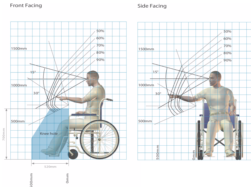
Figure 9 Reach and Viewing Angles (Wheelchair Users)
