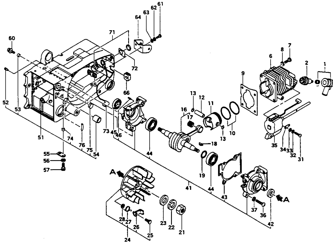
FIG. 1 ENGINE
