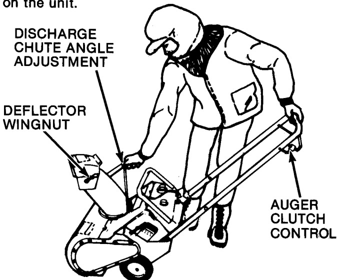
FIGURE 2 - DISCHARGE & BLOWER CONTROLS
