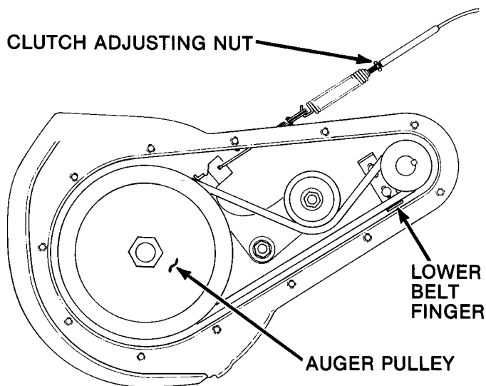
FIGURE 3 - AUGER CLUTCH-BELT ARRANGEMENT
