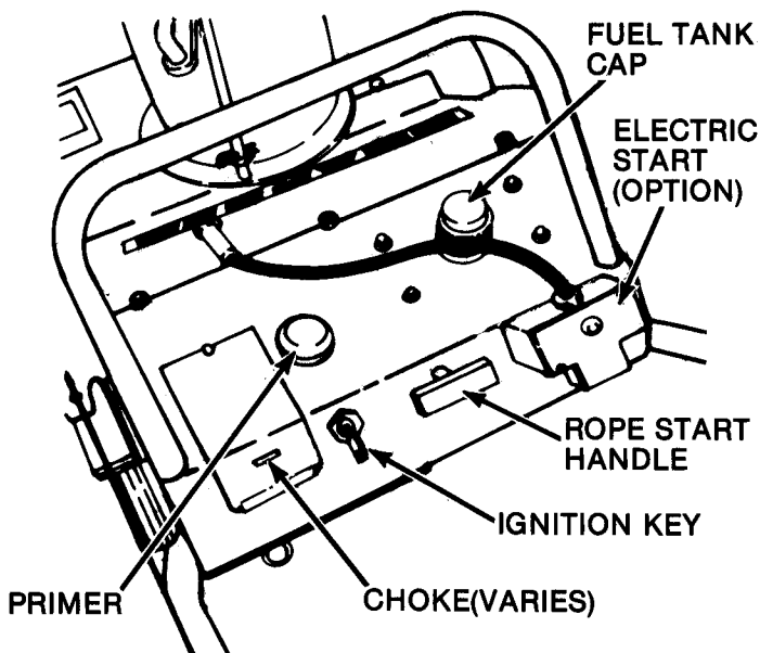
FIGURE 1 - LOCATION OF PANEL CONTROLS
