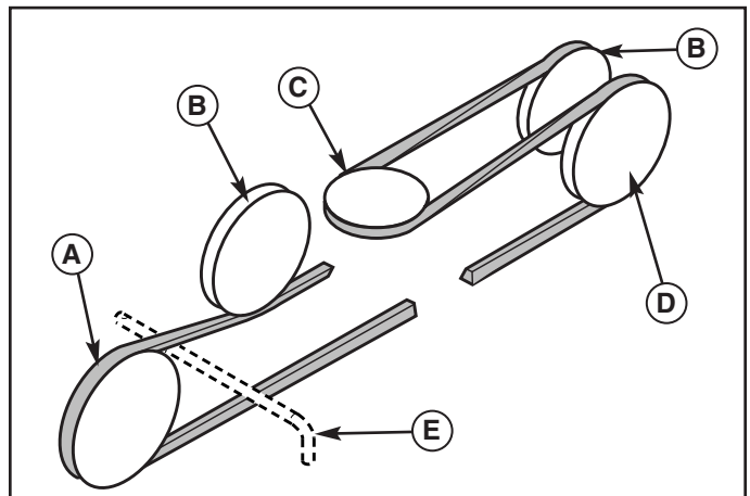
Figure 35. Belt Routing
