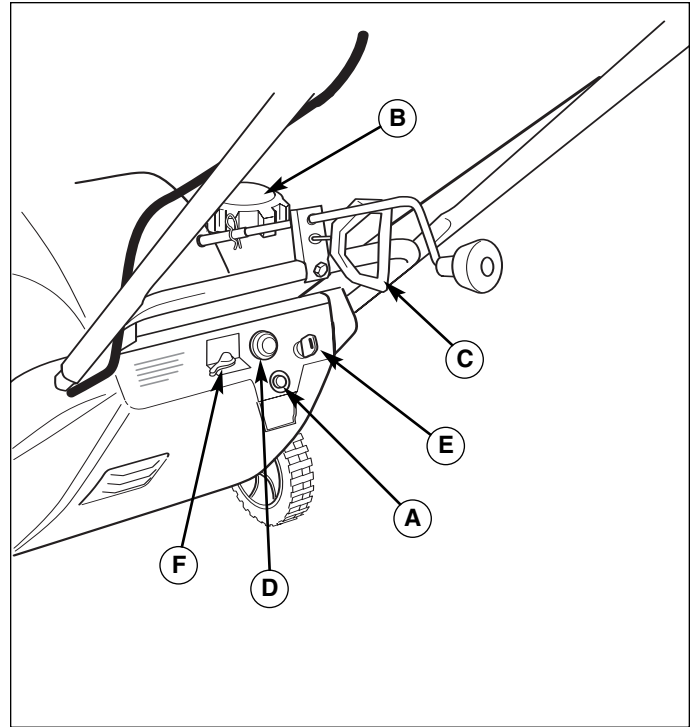
Figure 8. Engine Controls
