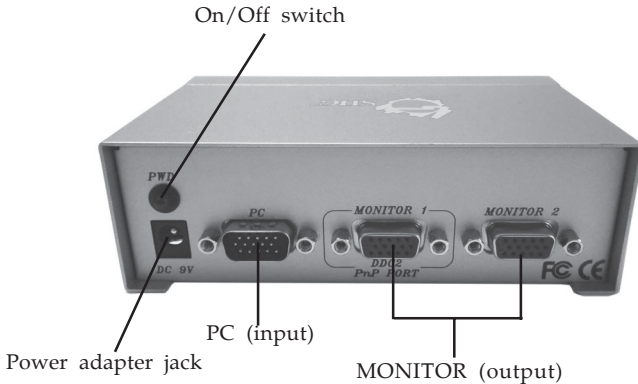
Figure 1: Rear Panel
