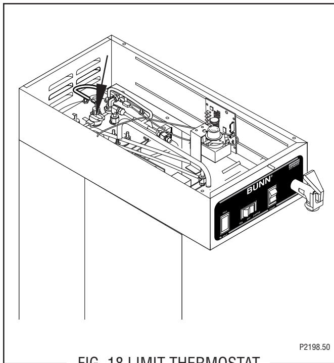
FIG. 18 LIMIT THERMOSTAT
