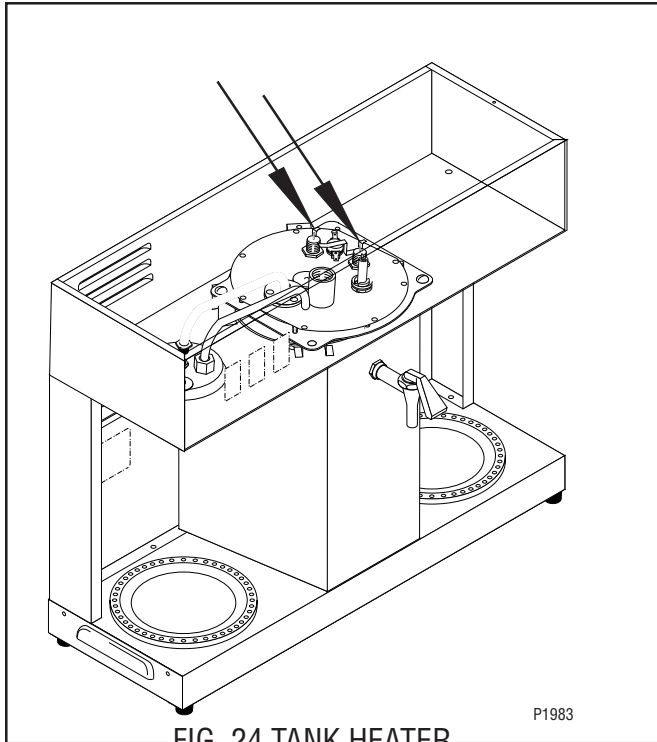
FIG. 24 TANK HEATER
