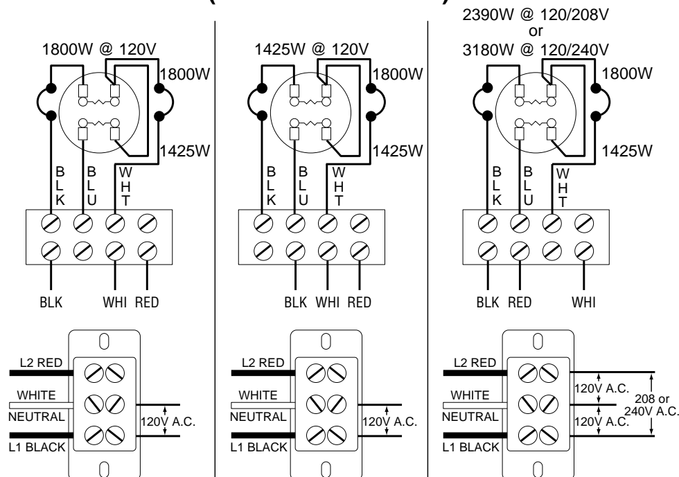
FIG. 9 TANK HEATER TO TERMINAL BLOCK WIRING
