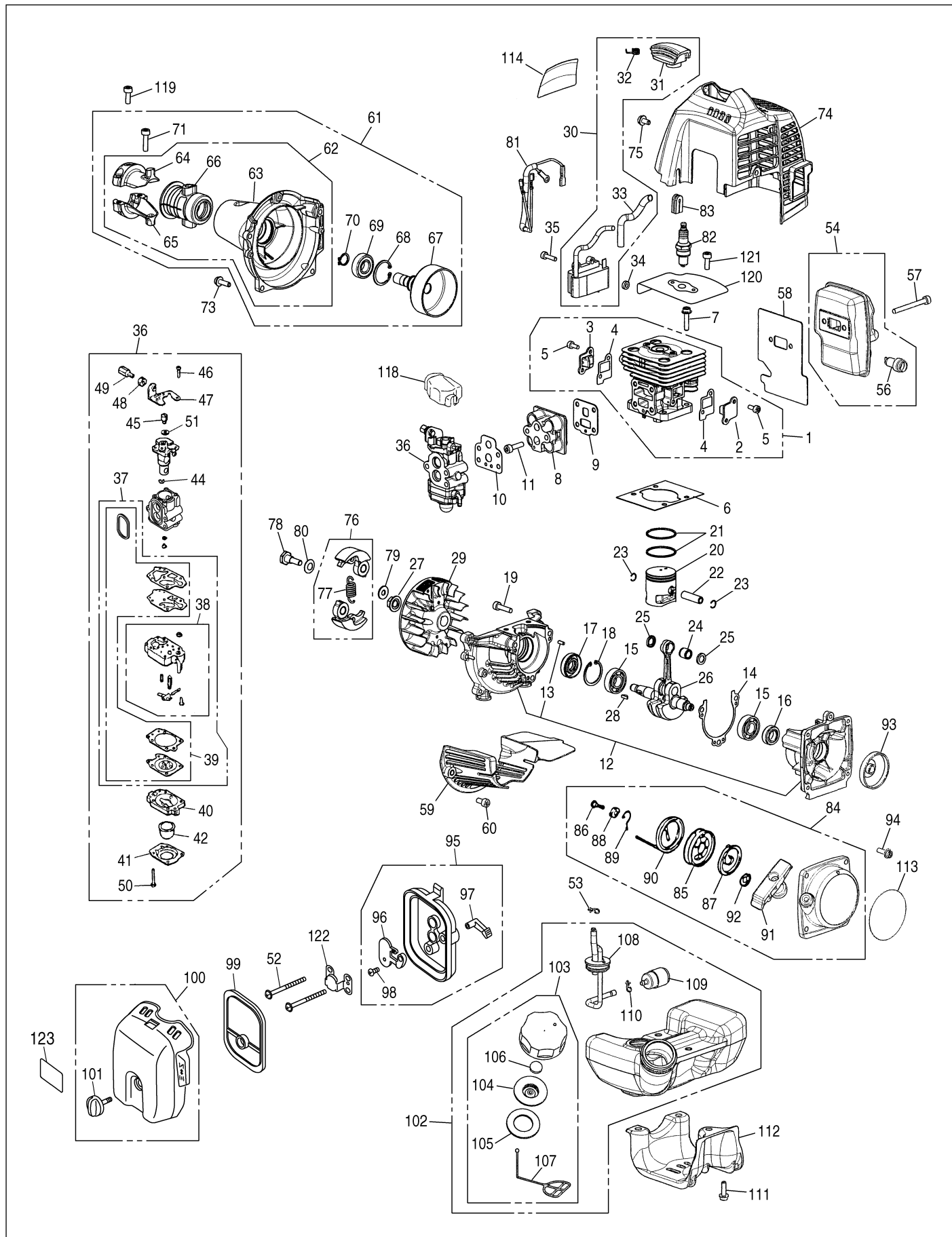
Fig.3 ENGINE UNIT BCZ2450S/T (S/N 90200101 and up)
