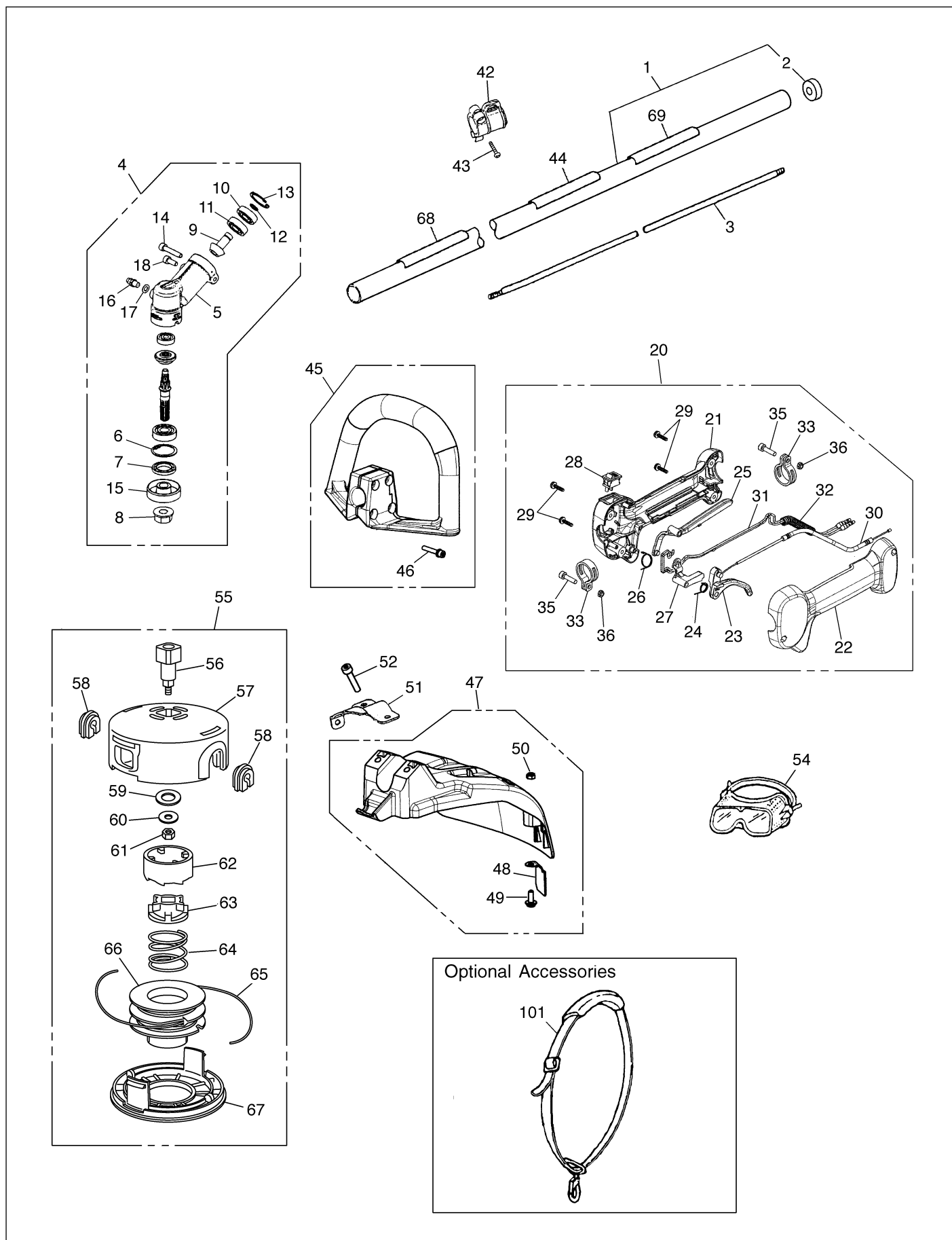
Fig.2 DRIVE UNIT BCZ2450T (S/N 90200101 and up)
