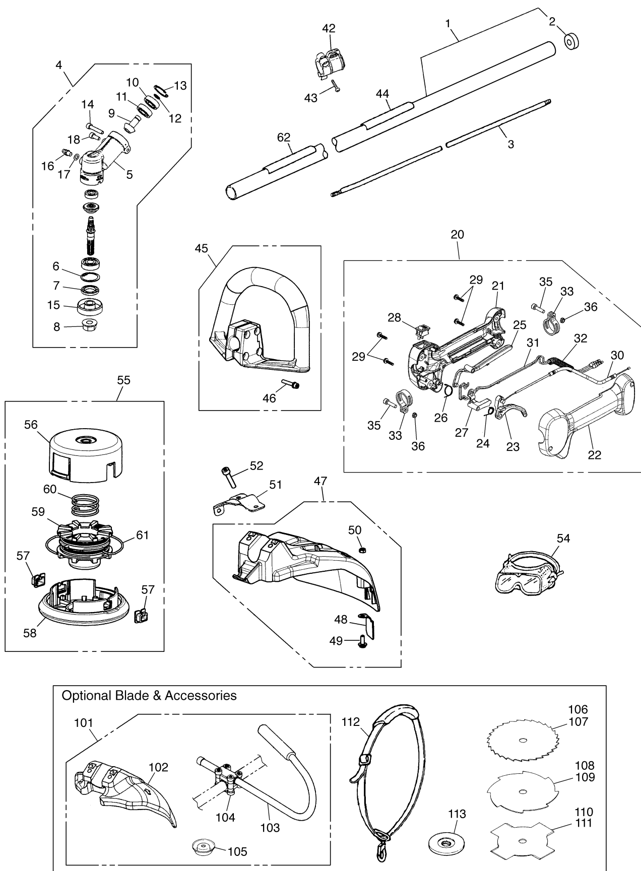
Fig.1 DRIVE UNIT BCZ2450S (S/N 90200101 and up)
