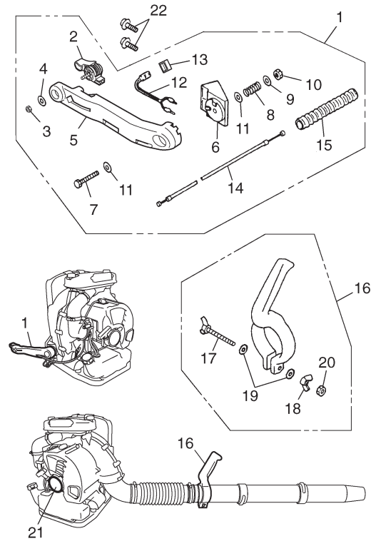
Fig.4 LEVER SET [EBZ8000]
