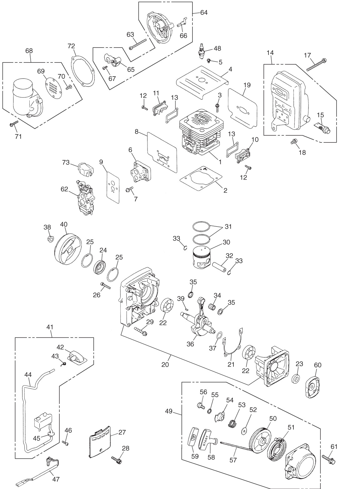
Fig.2 ENGINE GROUP (S/N 40500101 and up)
