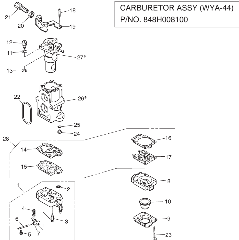
Fig.3 CARBURETOR COMPONENTS (S/N 40500101 and up)
