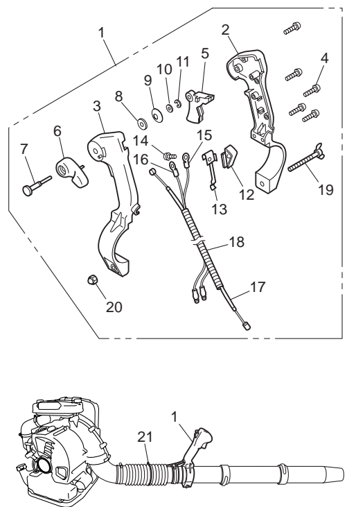
Fig.5 LEVER (R) SET [EBZ8000RH]
