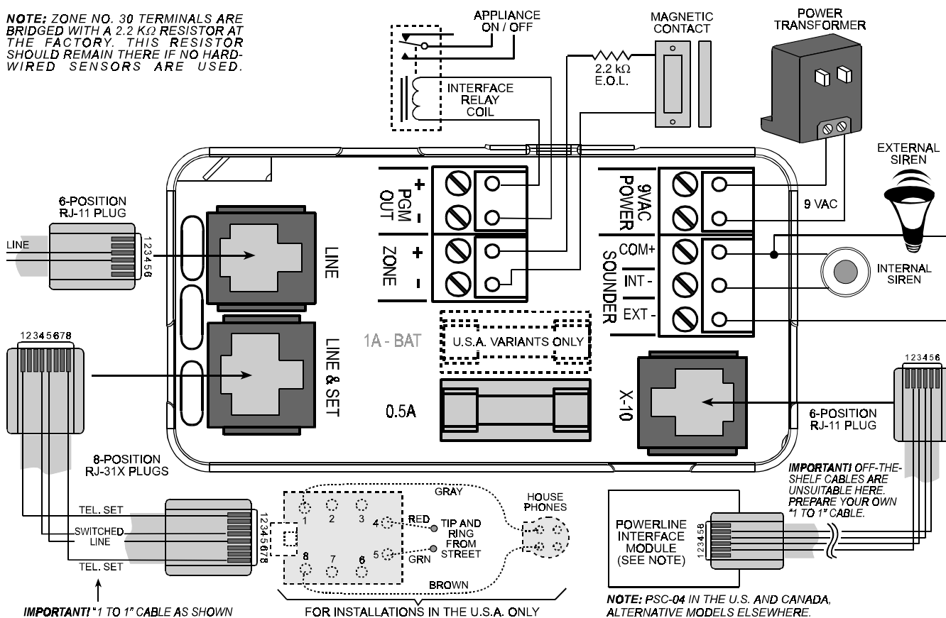
Figure 10. Wiring Diagram
