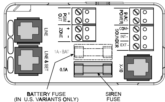
Figure 32. Fuse Locations
