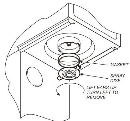
Fig. 11 Cleaning
