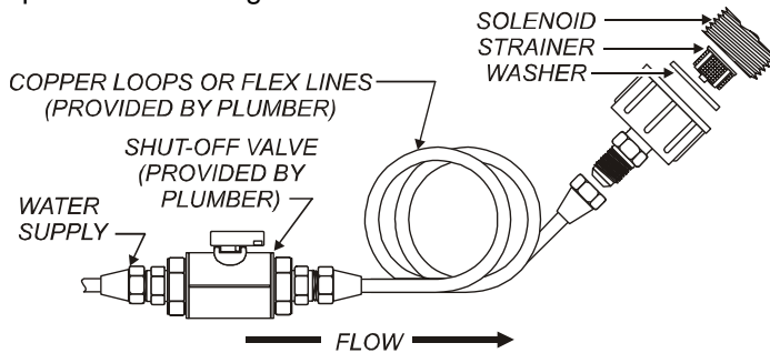
Fig. 2 Water Supply Installation
