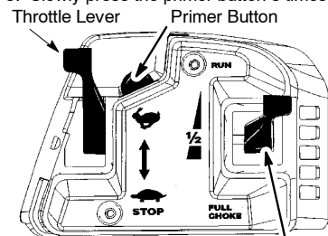
Choke Lever
