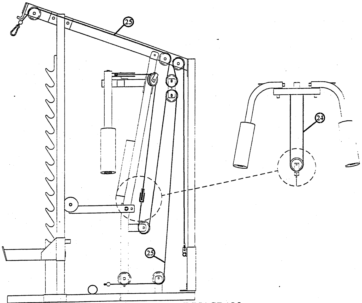
893103 CABLE DIAGRAM
